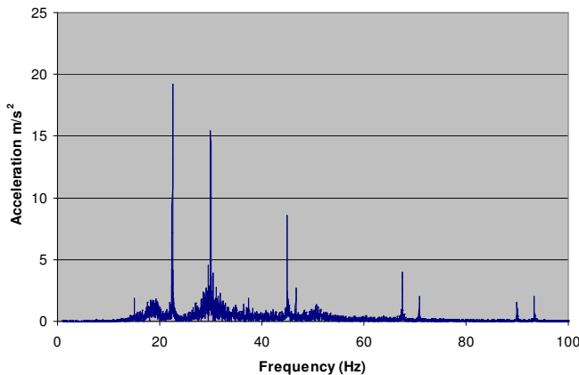
Fig. 1: Vibration frequency spectra on a helicopter vertical stabilizer.
