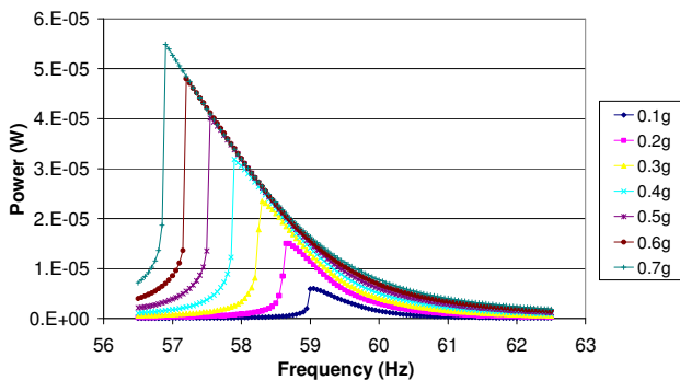
Fig. 4: 59Hz generator (30Hz design) power output
