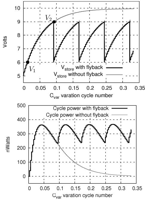
Figure 3: Example of operation of the conditioning circuit with and without flyback (thick and thin lines respectively). Top: V_{store} evolution, bottom: evolution of the average power harvested during one C_{var} variation cycle.
