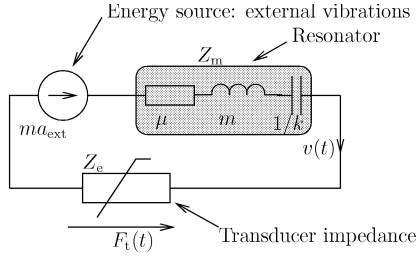
Figure 2: Equivalent electrical network of the harvester.
