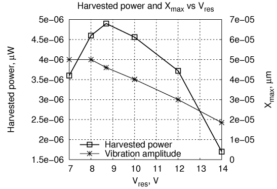
Figure 5: Modeling results: vibration amplitude and harvester power with V_{store} = 20.8\ \text{V} ( V_1 = 20\ \text{V} , V_2 = 21.6\ \text{V} ).
