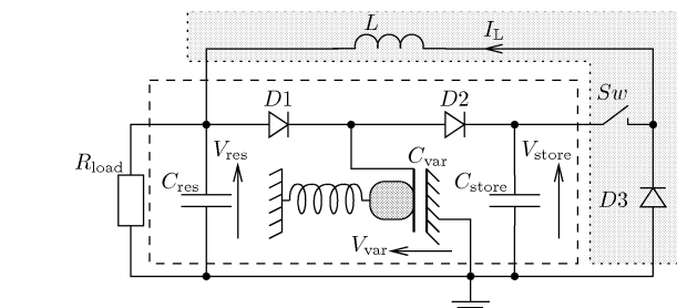
Figure 1: Electrical scheme of the harvester.
